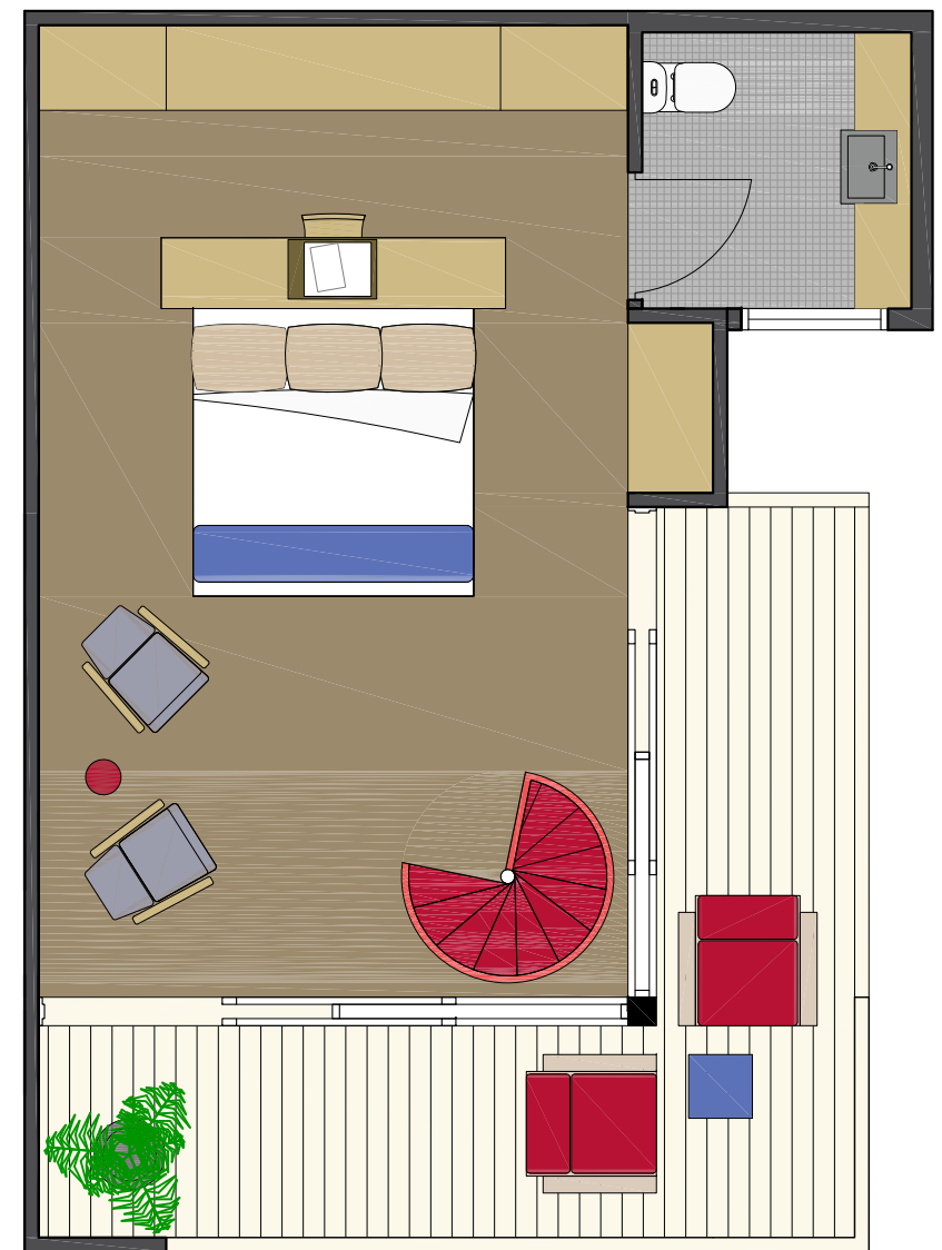
UPPER LEVEL FLOOR PLAN
